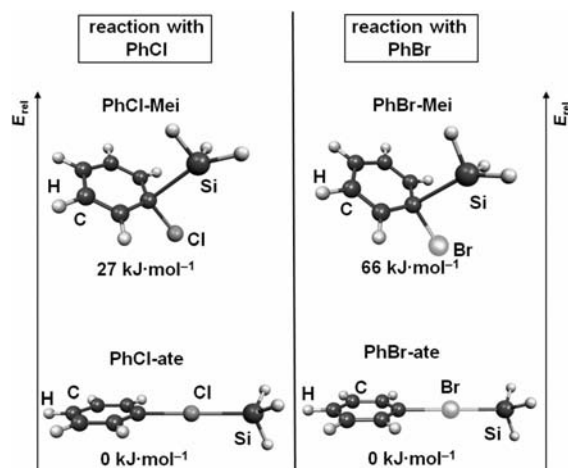
Figure 3. Calculated stationary points for the studied model systems H 3 Si-/PhCl (left) and H 3 Si-/PhBr (right) [B3LYP/6-31+G(d), CPCM]; in both cases, an ate complex and a reaction via an intermediate analogous to a Meisenheimer complex were optimized; Molekel plots. [36]
